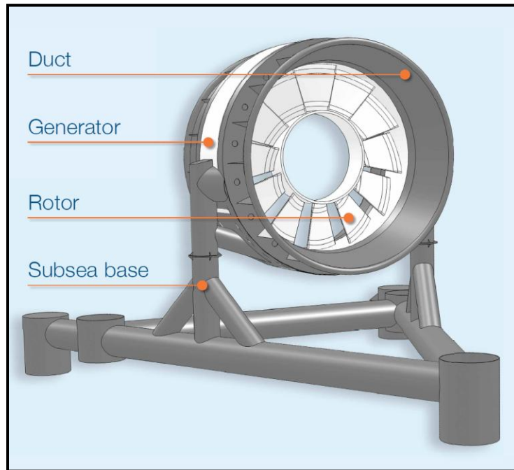
FIGURE 2-2 OPENHYDRO TURBINE 3
