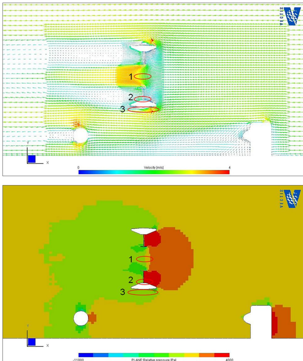
FIGURE 5-6 CFD SIMULATION OF VELOCITY VECTORS AND PRESSURES THROUGH AND AROUND THE TURBINE IN 2.5 M/S FLOW
