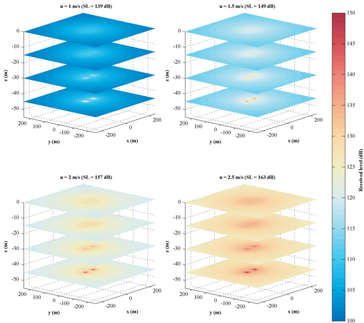
FIGURE 5-9 RECEIVED BROADBAND SOUND PRESSURE LEVELS AT CLOSE RANGE TO THE PROJECT AT VARIOUS DEPTHS
