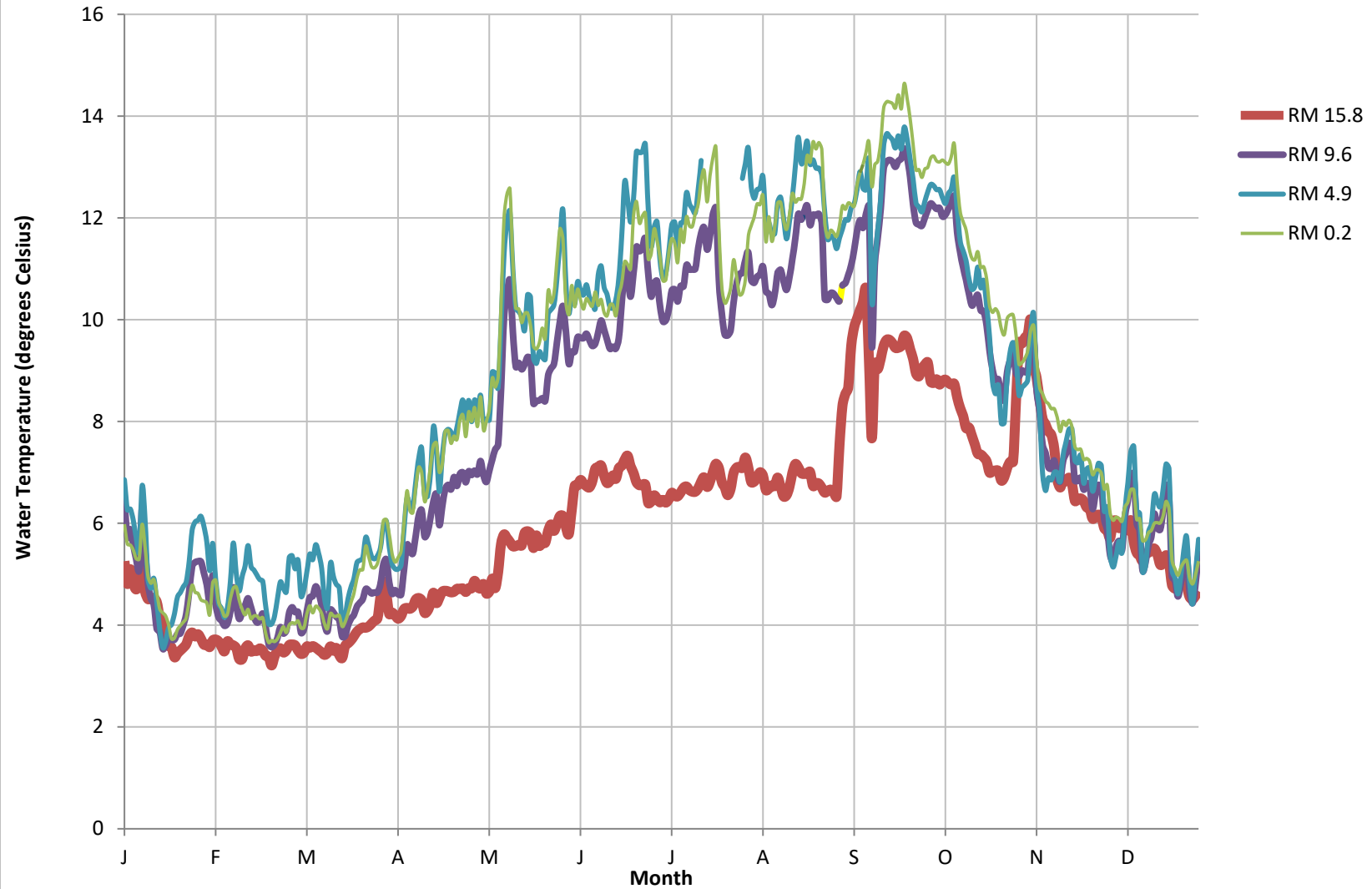
Figure A-3. Longitudinal Depiction of Mean Daily Water Temperature, Sultan River downstream of Culmback Dam during 2020
