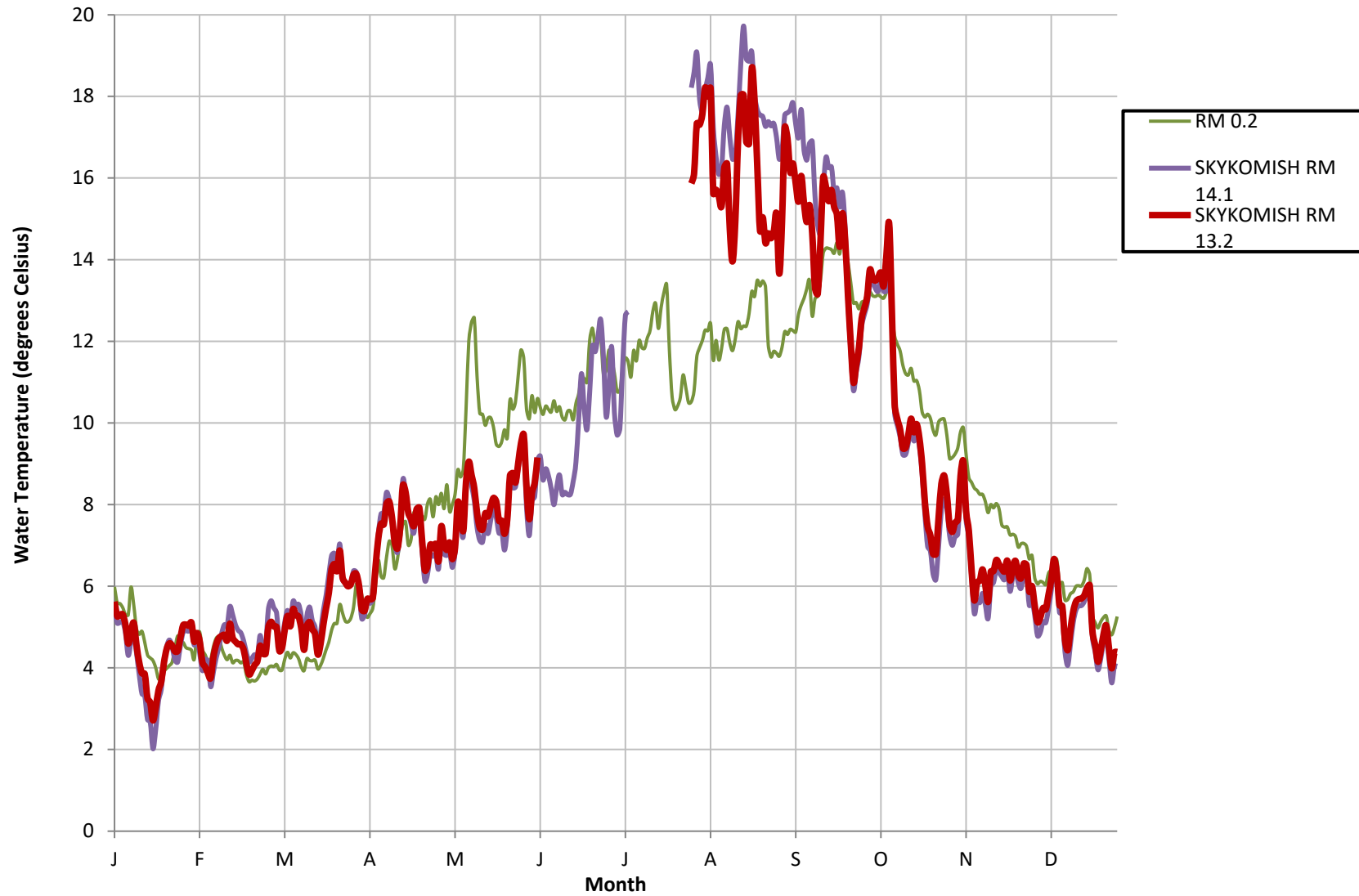
Figure A-4. Mean Daily Water Temperature near confluence of Sultan and Skykomish rivers during 2020
