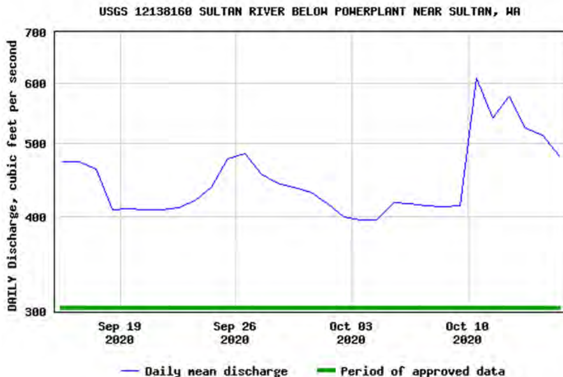
Figure 3. Mean Daily Discharge in the Sultan River downstream of the Powerhouse between September 15 and October 15, 2020.
