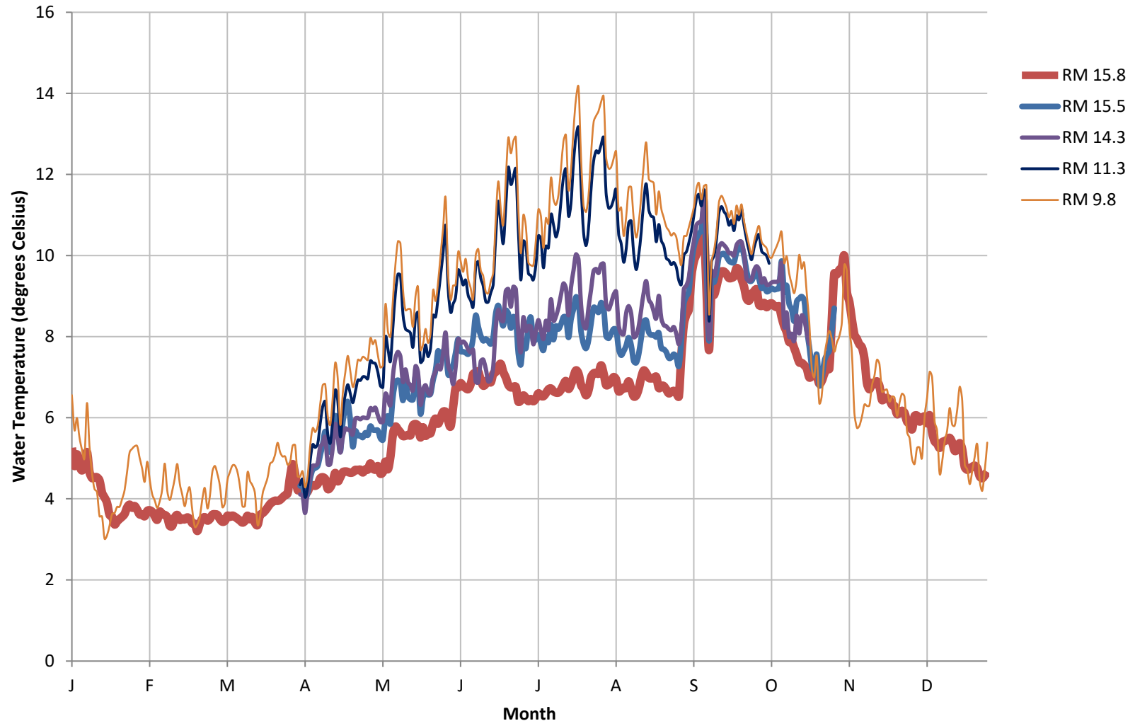
Figure A-2. Longitudinal Depiction of Mean Daily Water Temperature in the Bypass Reach (Reach 3) of the Sultan River during 2020
