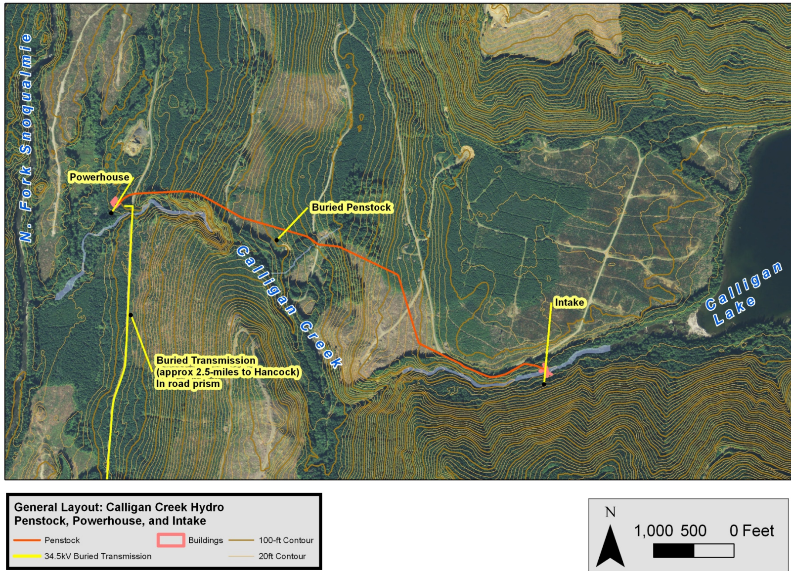
Figure 1-1. General Project layout: penstock, powerhouse and intake.
