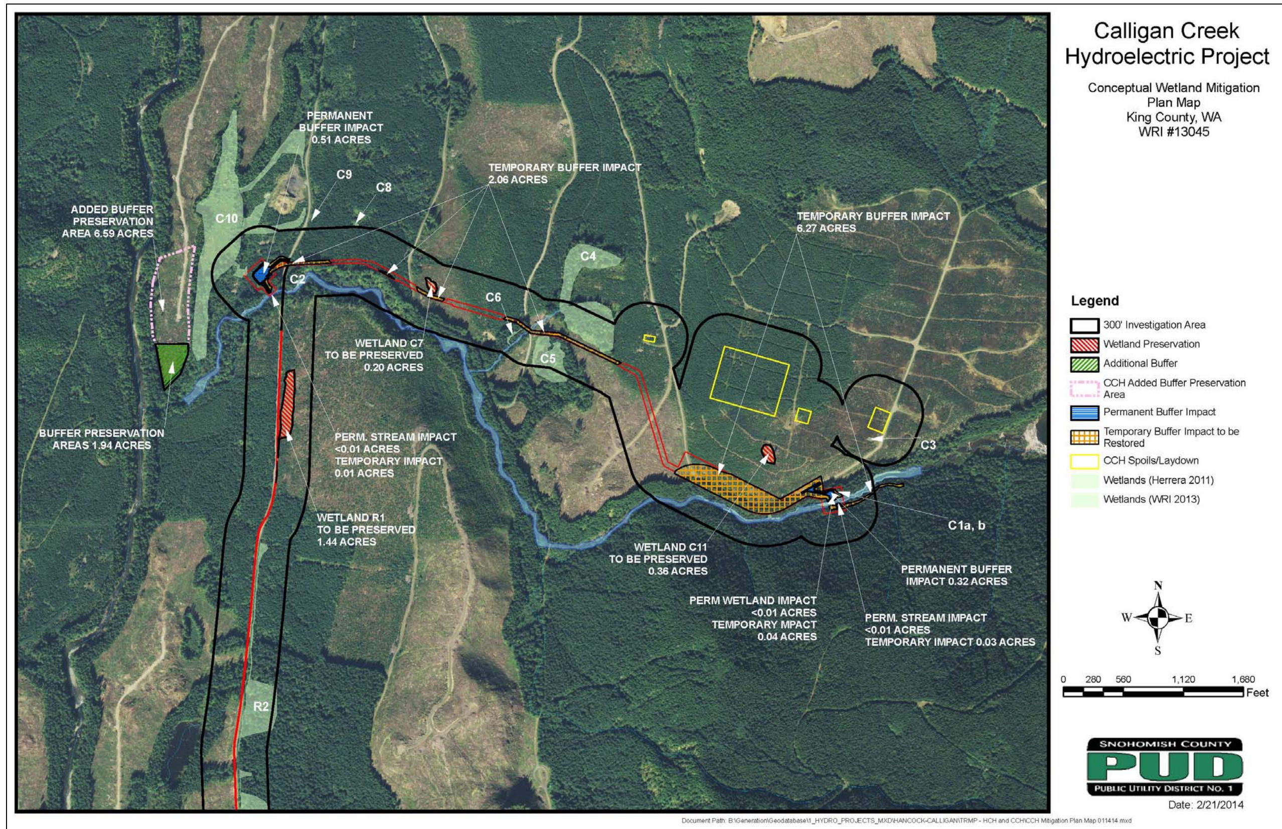
Figure 2-2. Wetland, stream and buffer mitigation.
