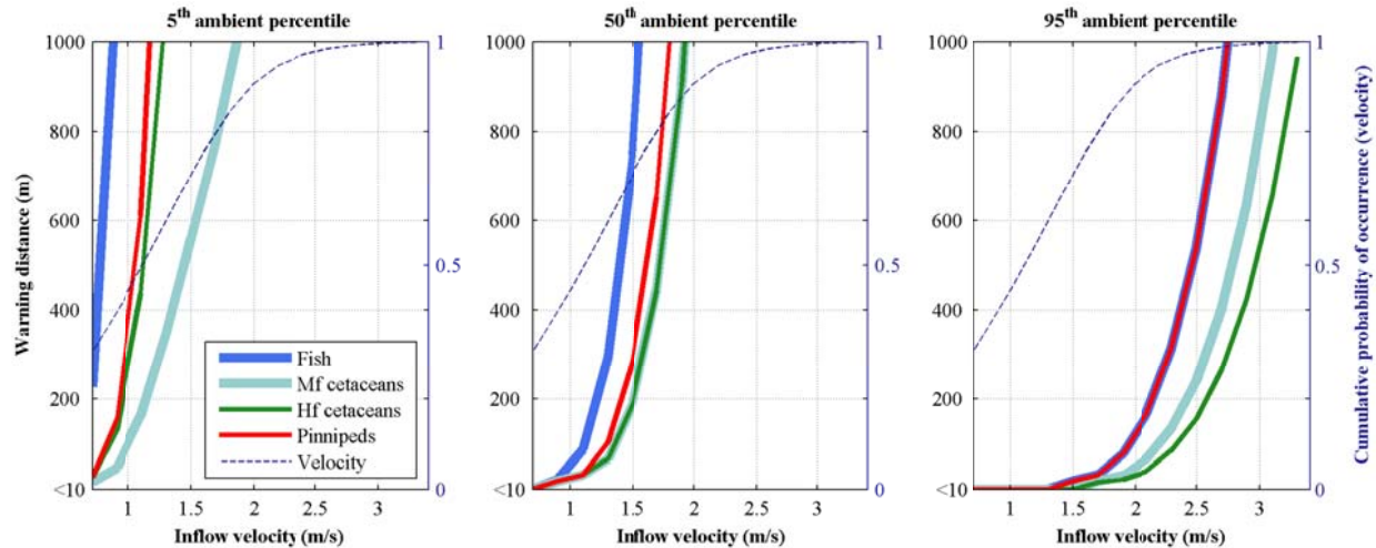
Figure 16 – Warning distance (30 m depth relative to surface) as a function of inflow velocity.
