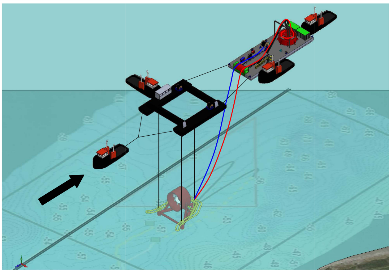
Figure 1: Baseline Installation
