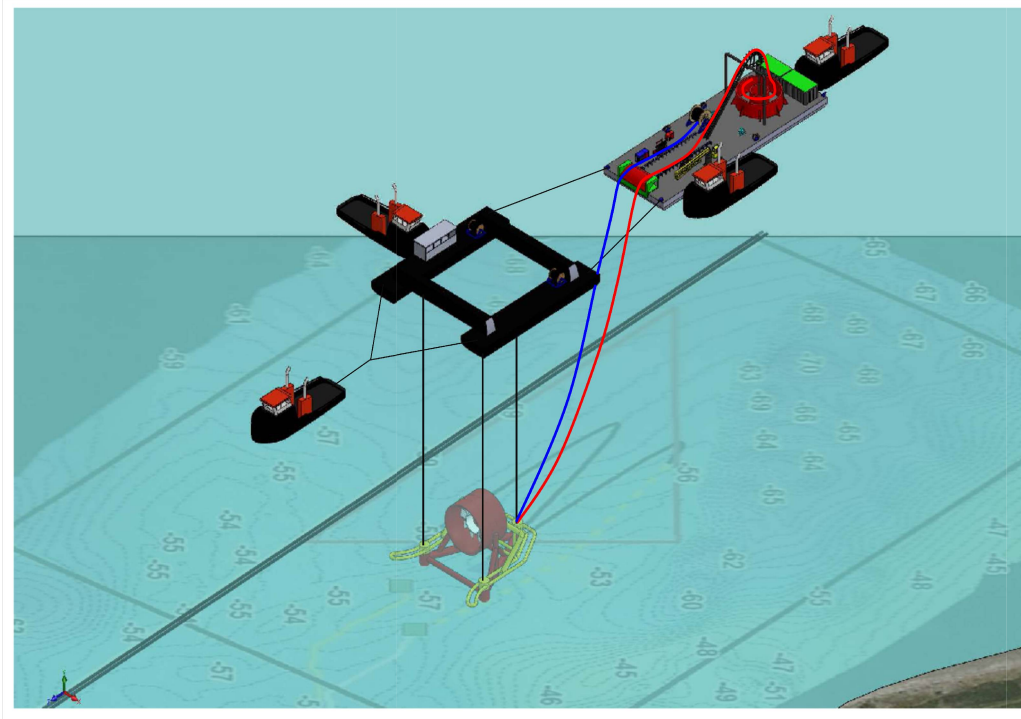
Figure 1 Installation Configuration
